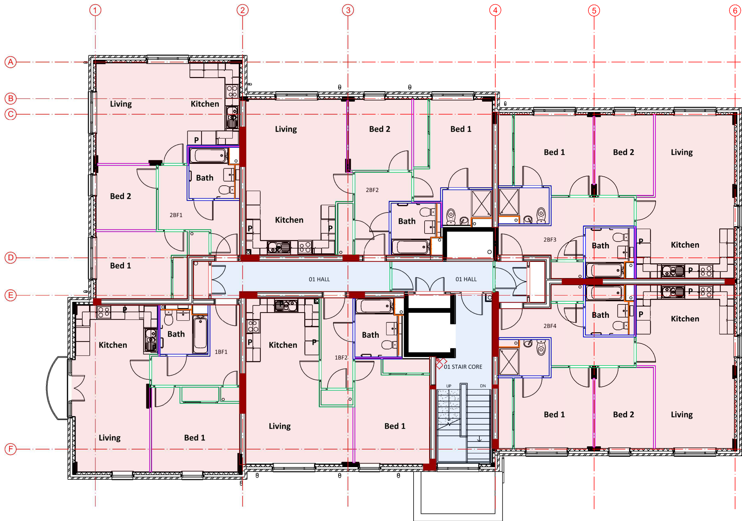
Proposed First/Second/Third Floor Plan
