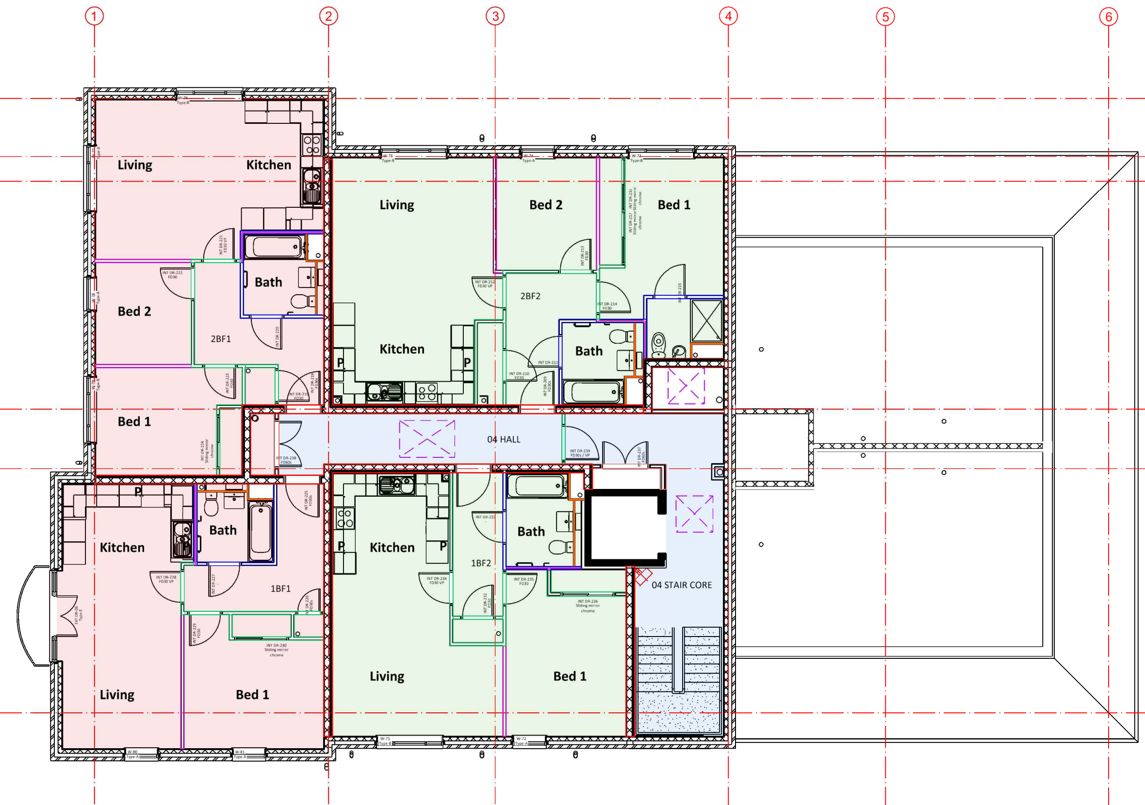
Proposed Fourth Floor Plan
