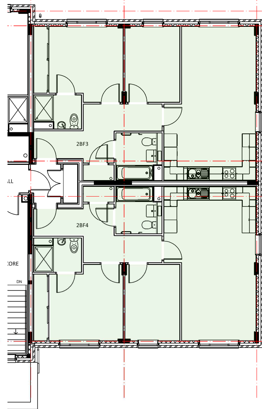
Top Floor 2BF3 & 2BF4 All walls as lower floors ceiling to be 30 minute fire rated
